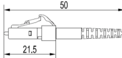
Patchcord
