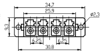
Quad SC-type
