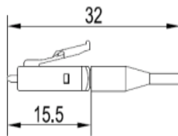
Pigtail
