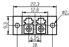
Duplex SC-type
